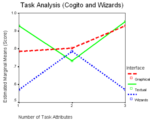
Figure 3: User task analysis comparing user task scores on the wizard and example-based (graphical and textual) interfaces.
