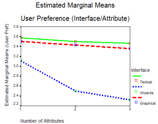
Figure 4: Graph showing the mean preference ratings for each interface, for each number of attributes. The textual and graphical example-based interfaces are rated consistently high, while the wizard interfaces are preferred less as the number of attributes increases.
