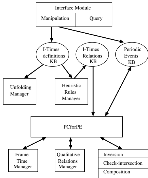
Figure 2: Architecture of the TeMP system
