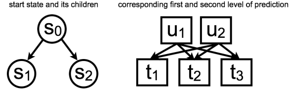
Figure 1: The first step of a CDP prediction for start state s_0 .
